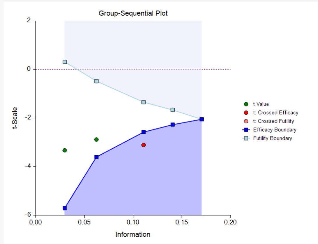
Group-Sequential Boundary Plot at Stage 3
