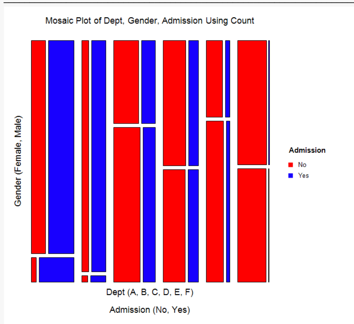
Mosaic Plot of Dept, Gender, Admission Using Count
